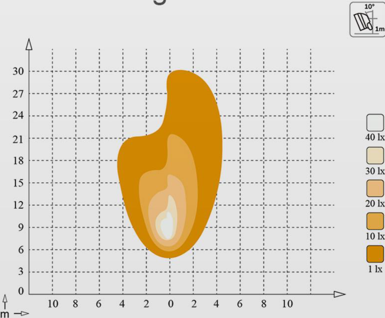
low beam
