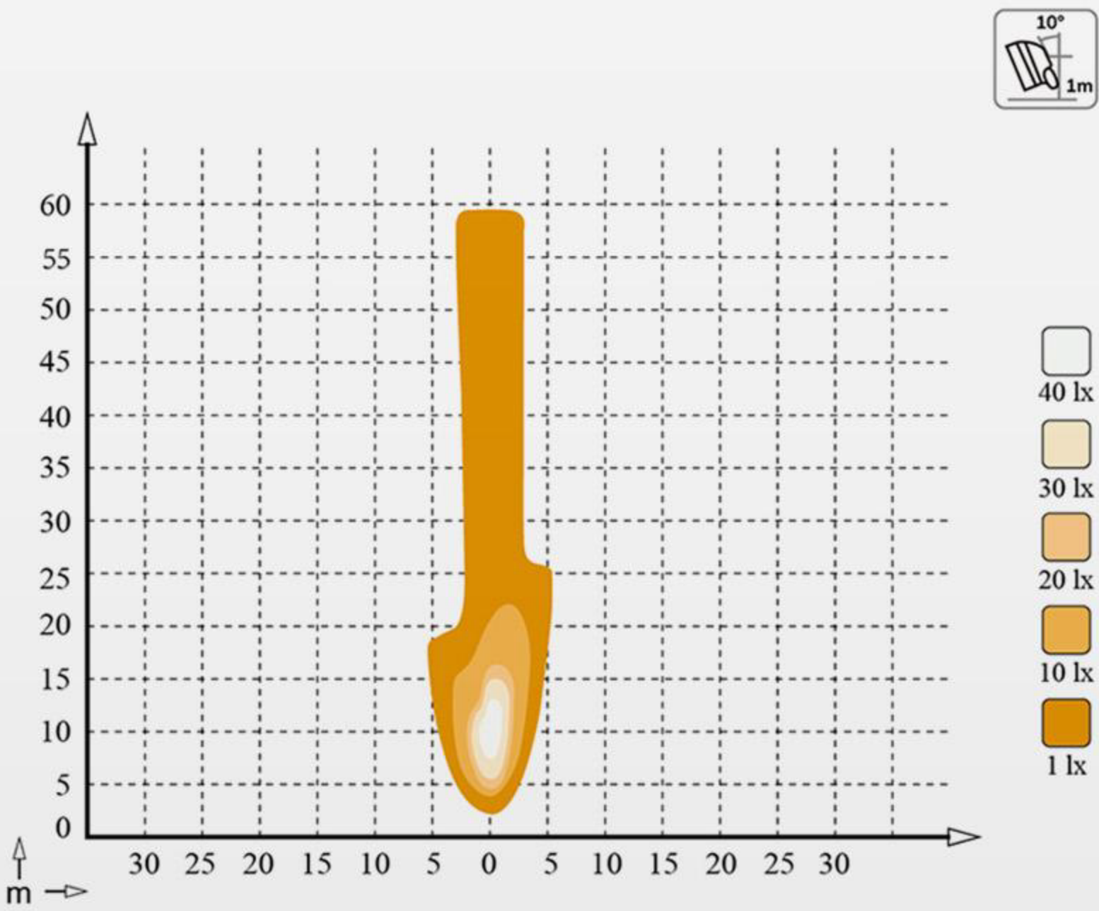
high beam
