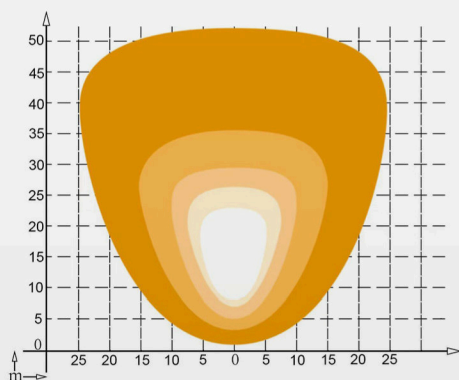
LED-flood
