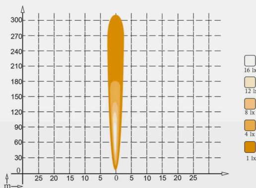
LED-SPOT
