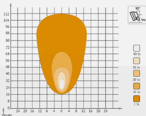
LED-flood
