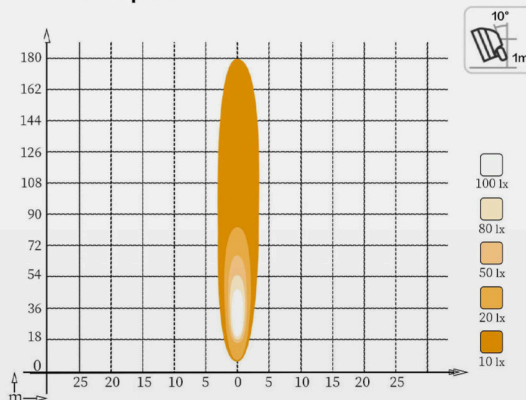
LED-spot
