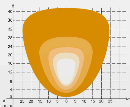
LED-flood
