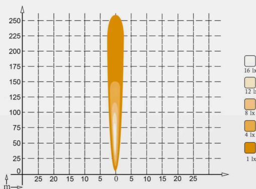
LED-SPOT
